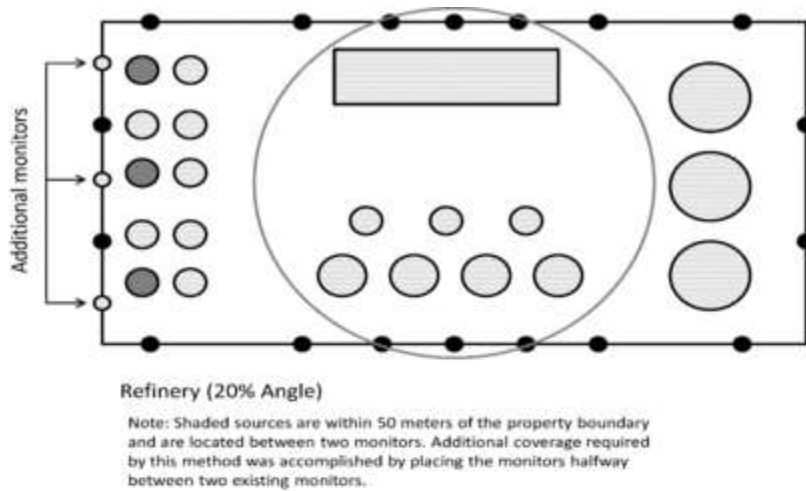
Figure 8.1. Facility with a Regular Shape Between 750 and 1,500 Acres in Area
