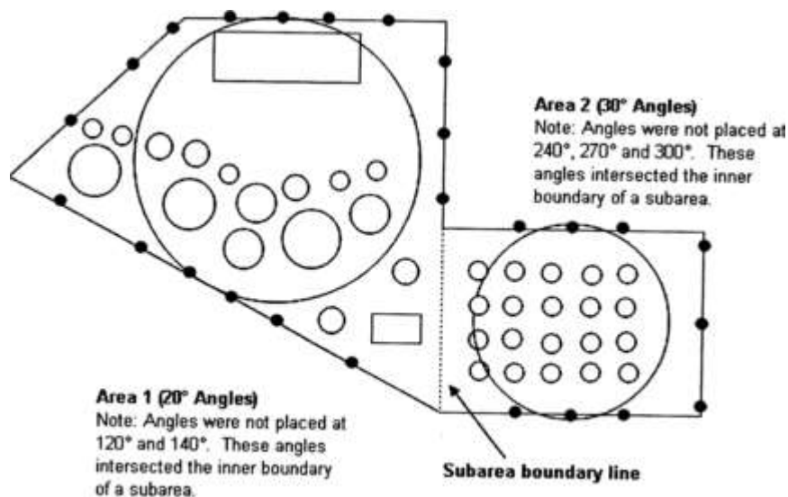
Figure 8.4. Facility Divided into Two Subareas
